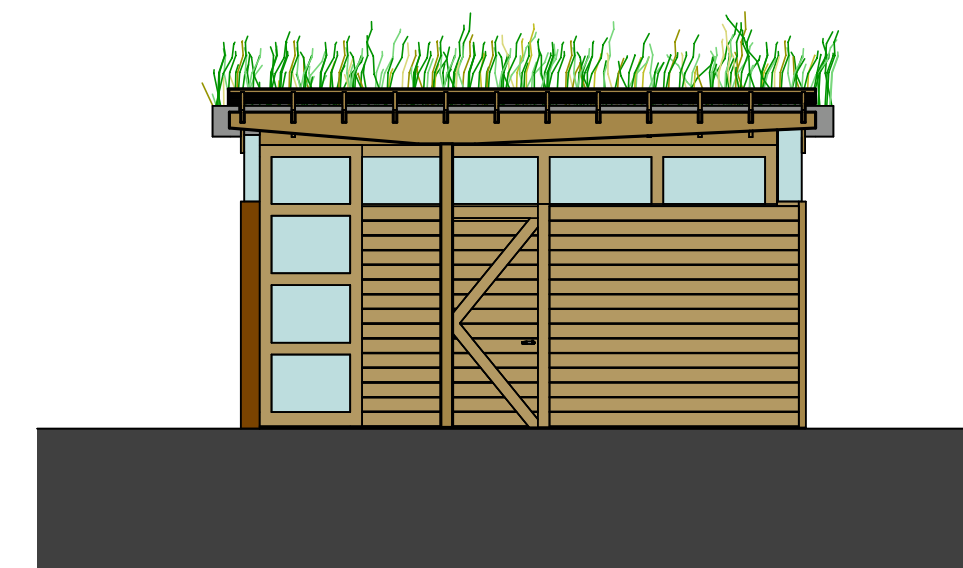
SOUTH ELEVATION
