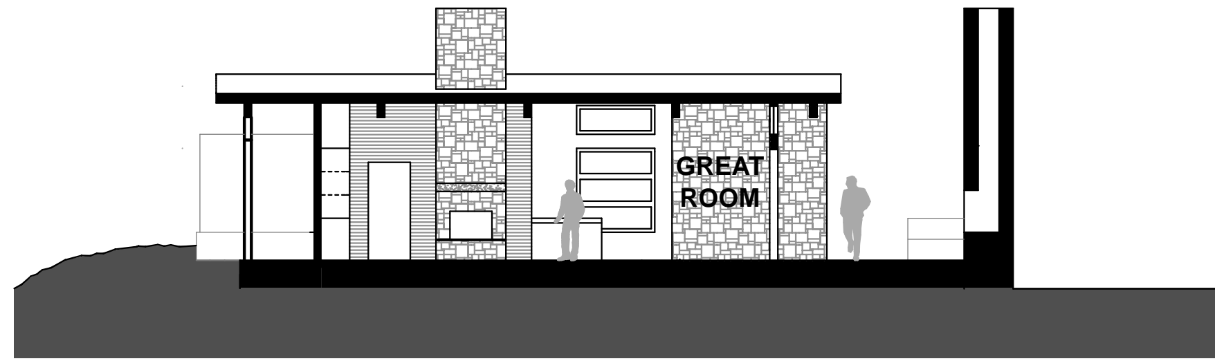
E/W SECTION
