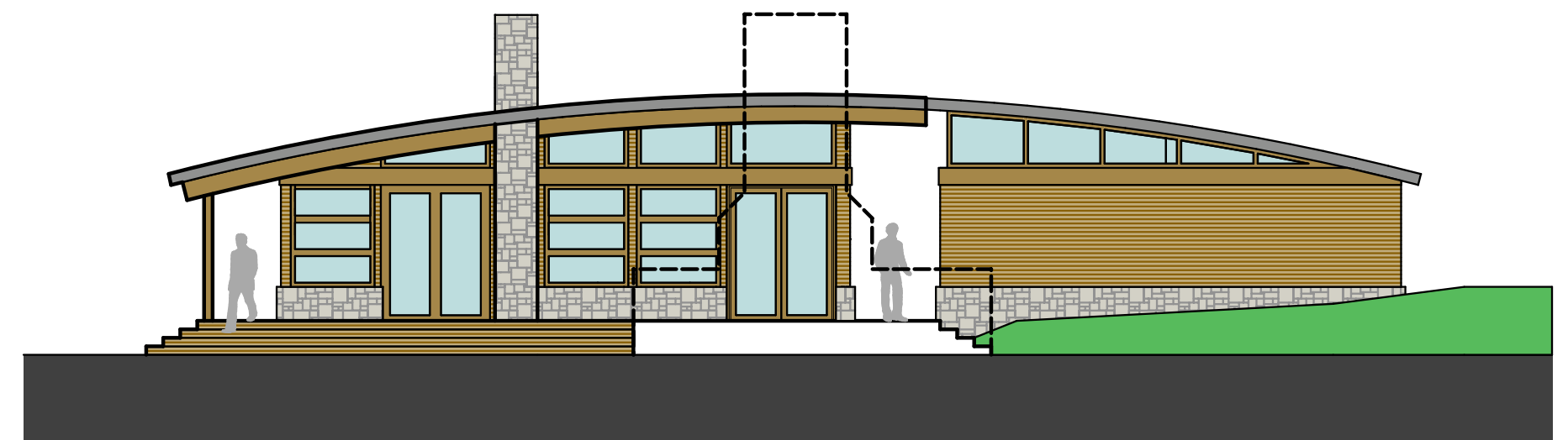
EAST ELEVATION
